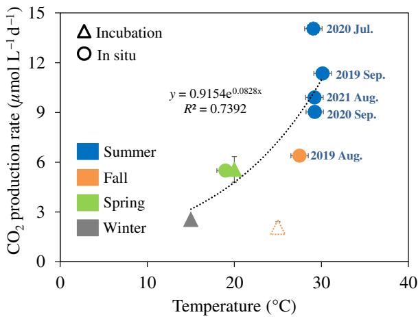
Fig. 6. Comparison of the relationship between CO_2 production rate based on incubations (triangles) and calculated from oxygen utilization (circles) and temperature in the hypolimnetic water column of SK reservoir. The fall incubation result (open triangle) was excluded from the regression analysis because a lack of organic substrate resupply might have limited respiration activity.
