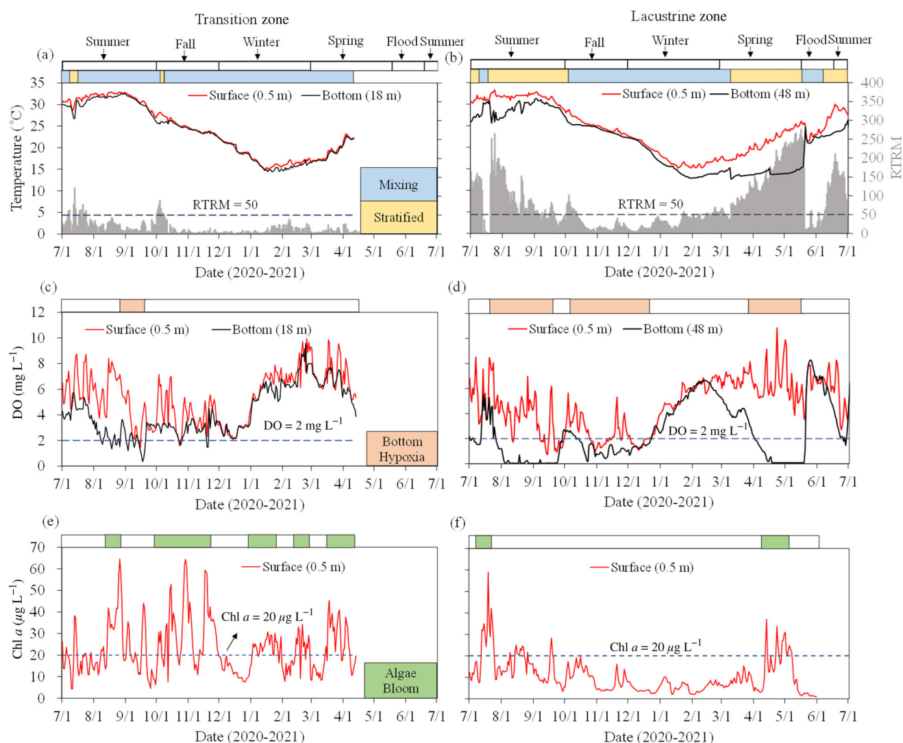
Fig. 1. Time-series data for surface and bottom temperature ( a, b ), DO ( c, d ), and surface Chl a ( e, f ) in transition and lacustrine zones (Z3 and S4) of SK reservoir. A stratification index RTRM (relative thermal resistance to mixing, gray shaded) of 50 was used to divide stratified vs. mixed periods in the reservoir. Bottom DO < 2 mg L -1 was defined as hypoxia and Chl a > 20 µg L -1 represents the algae bloom events.
